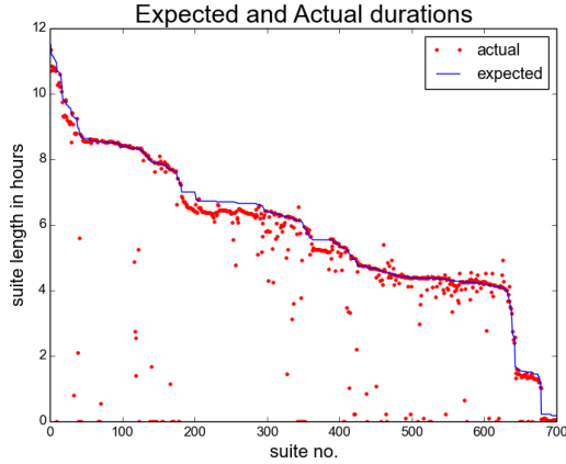
Fig. 3. Actual and expected durations of suites.
