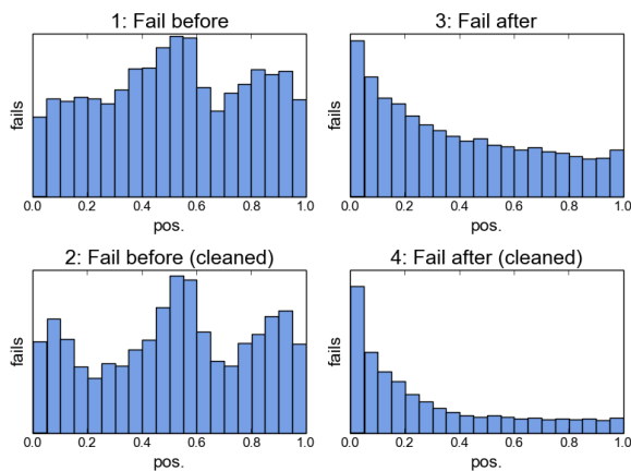
Fig. 5. Normalized fail distributions before and after the introduction of SuiteBuilder. The top row includes all test suites. In the bottom row, short and broken suites have been removed from the data set.
