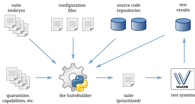
Fig. 2. Overview of the workflow of the SuiteBuilder tool.
