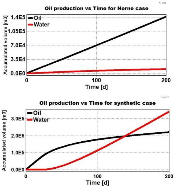
Figure 9. Accumulated oil and water production from Norne well and synthetic well
