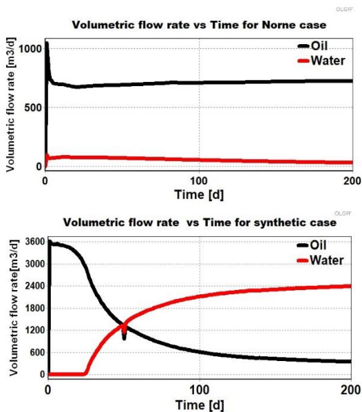
Figure 10. Volumetric flow rates of oil and water for Norne well and synthetic well
