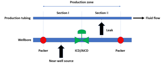
Figure 8. Simplified representation of a single production zone (Moradi et al, 2020).
