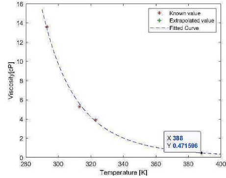
Figure 1. Extrapolated value of viscosity at reservoir conditions by curve-fitting
