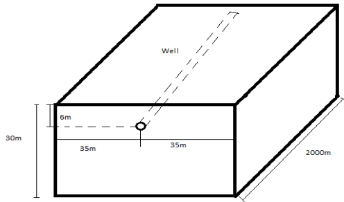
Figure 6. Location of well in drainage area of reservoir
