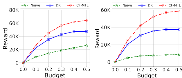
(a) Reward on YELP with coupon incentives.
