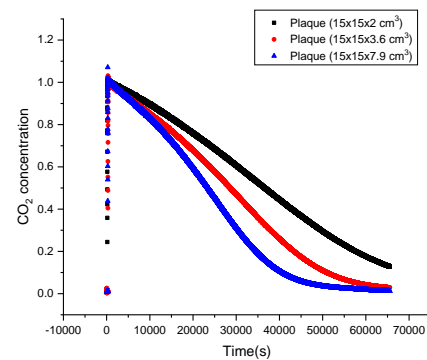
Figure 5. The curves show the dependence of the speed of carbonation of mortar to its external area exposed to the CO 2 of the chamber.
