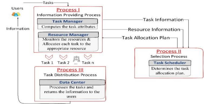
Figure. 12 The figure shows that task scheduling is divided into three processes
