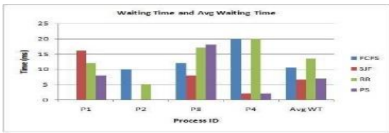
Figure 17: Comparison of Fundamental scheduling Algorithm-waiting Time
