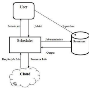
Fig4[11]Scheduling in cloud computing
