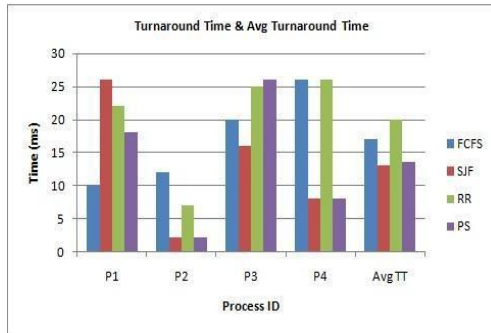
Figure 18: Comparison of Fundamental scheduling Algorithm-Turnaround Time
