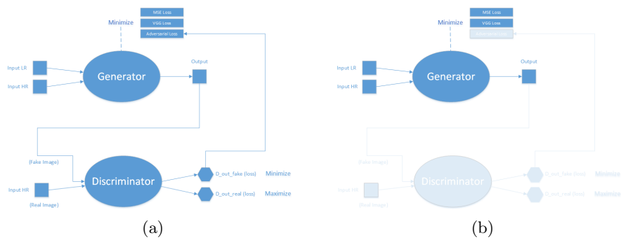
Fig. 2: (2a): SRGAN diagram, (2b): GFE, the proposed architecture – many of the elements go away
