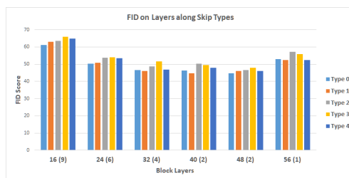
Fig. 9: Lower the better. (Numbers in parentheses indicate batch size)
