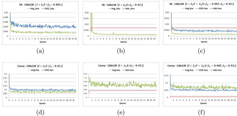
Fig. 4: Loss values by epochs from Figure 3a [ 128 \times 128 ] (a) I+V (b) I+A (c) I+V+A, and Loss values from Figure 3b [ 128 \times 128 ] (d) I+V (e) I+A (f) I+V+A
