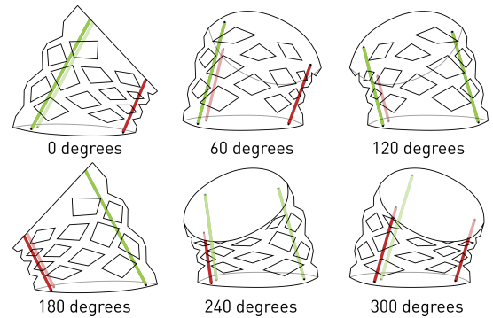
Fig. 2: The activation of a specific tendon pattern causes bending in one direction. For each combination, agonist (red) and antagonist (green) tendons can be identified. The six possible combinations of actuation that produce omnidirectional bending for a single module are shown.
