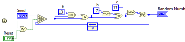
Fig. 2. Labview implementation of the 64bit Xorshift pseudorandom number generator.
